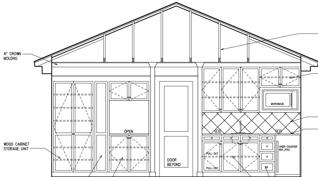
INTERIOR ELEVATION AT KITCHENETTE
