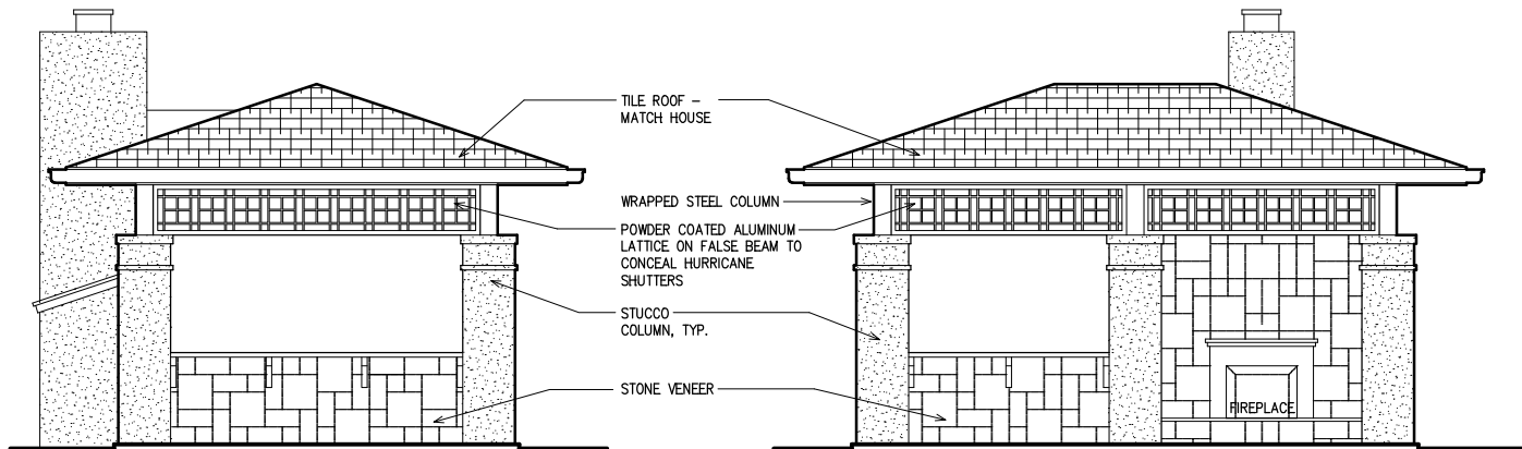
SOUTH ELEVATION
