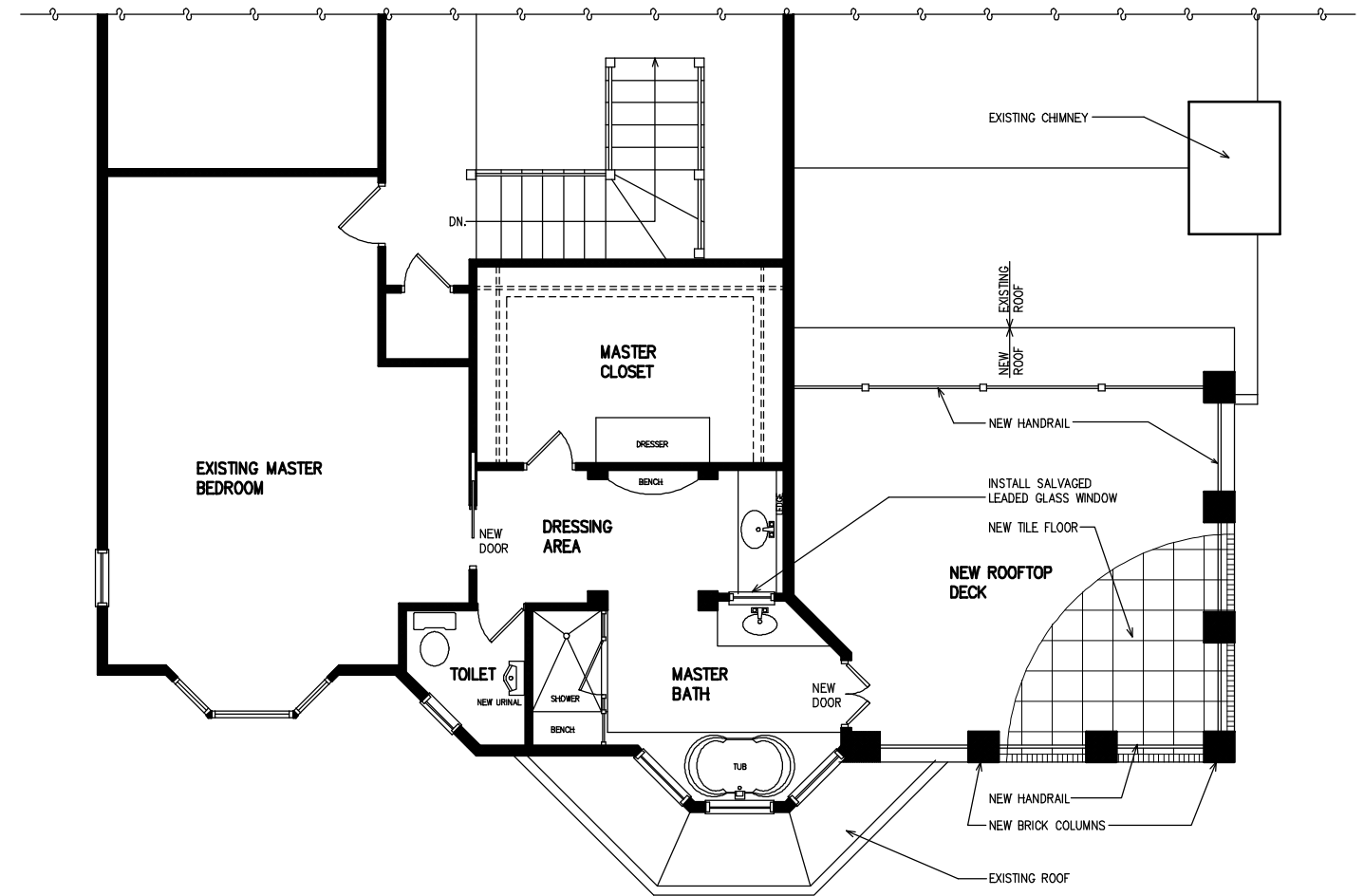
NEW SECOND FLOOR PLAN © COPYRIGHT 2008
