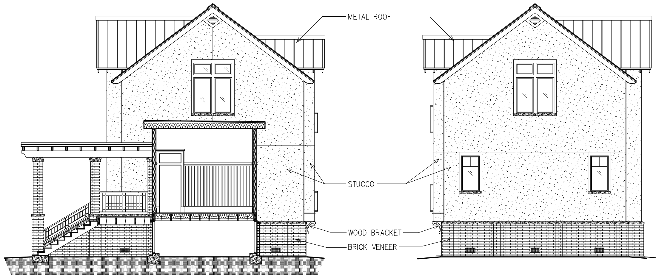
RIGHT SIDE ELEVATION / SECTION
